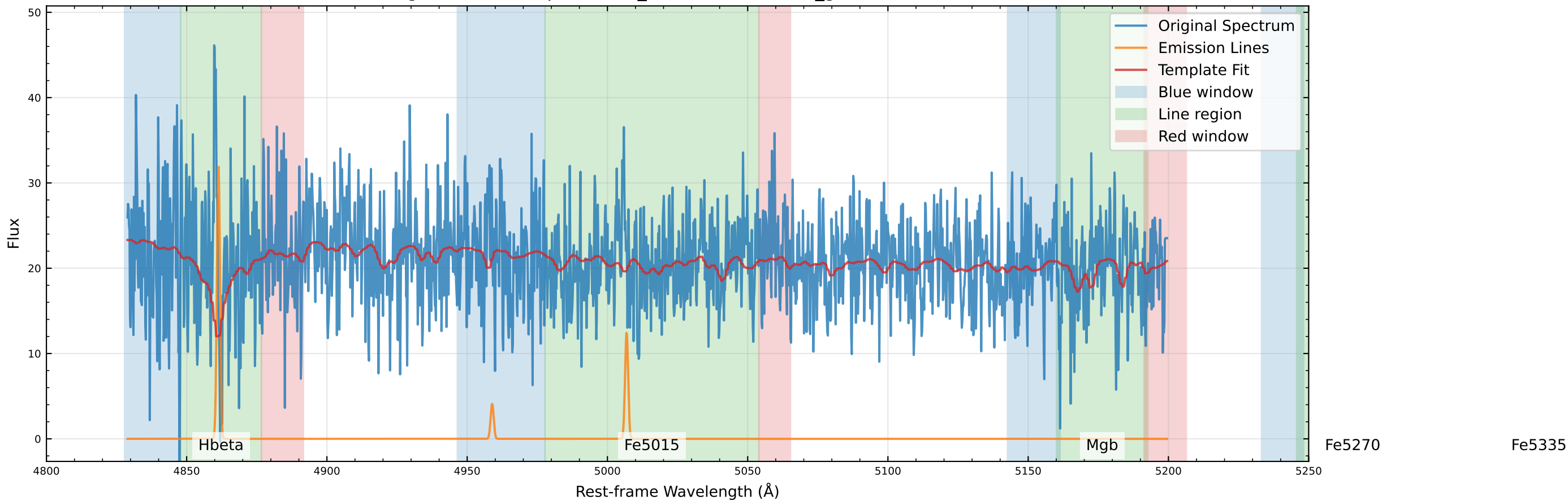
Original Data Comparison (v_star=-87.2 km/s, v_gas=-74.4 km/s)
