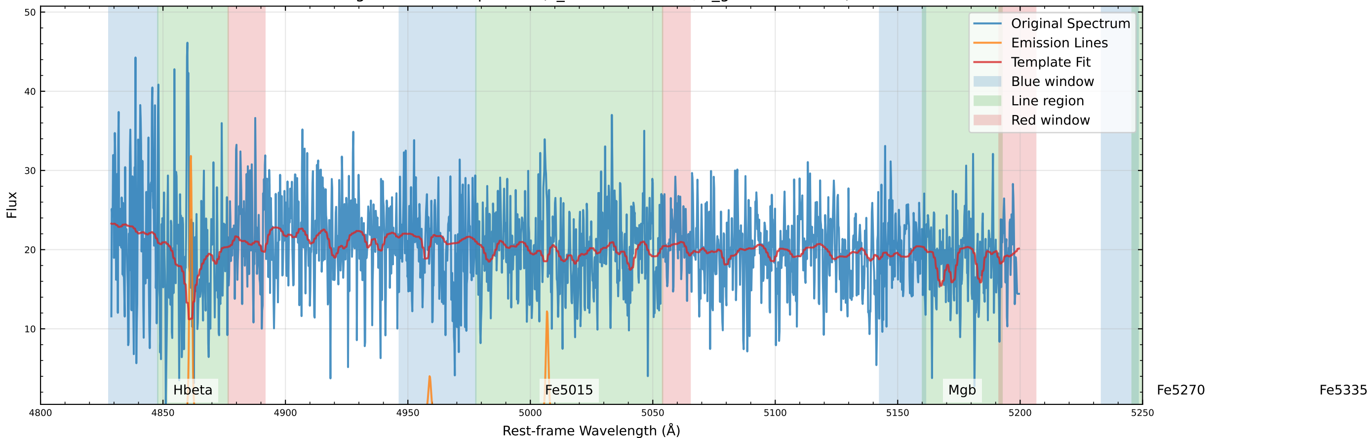
Original Data Comparison (v_star=-88.6 km/s, v_gas=-75.5 km/s)
