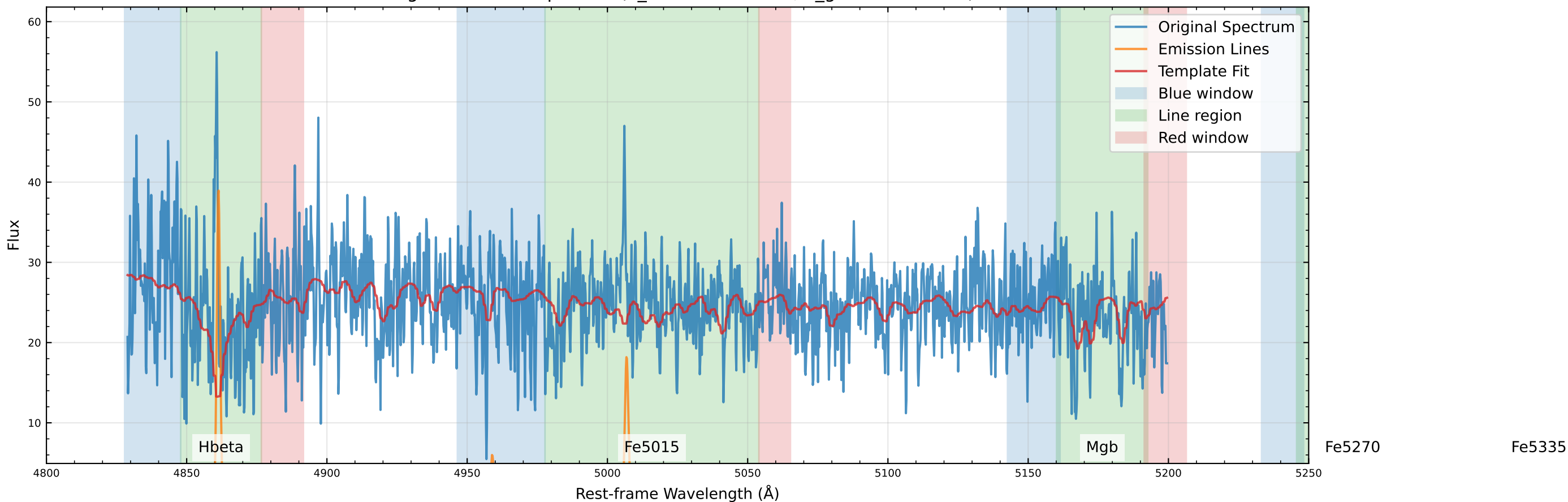
Original Data Comparison (v_star=-46.8 km/s, v_gas=-50.9 km/s)
