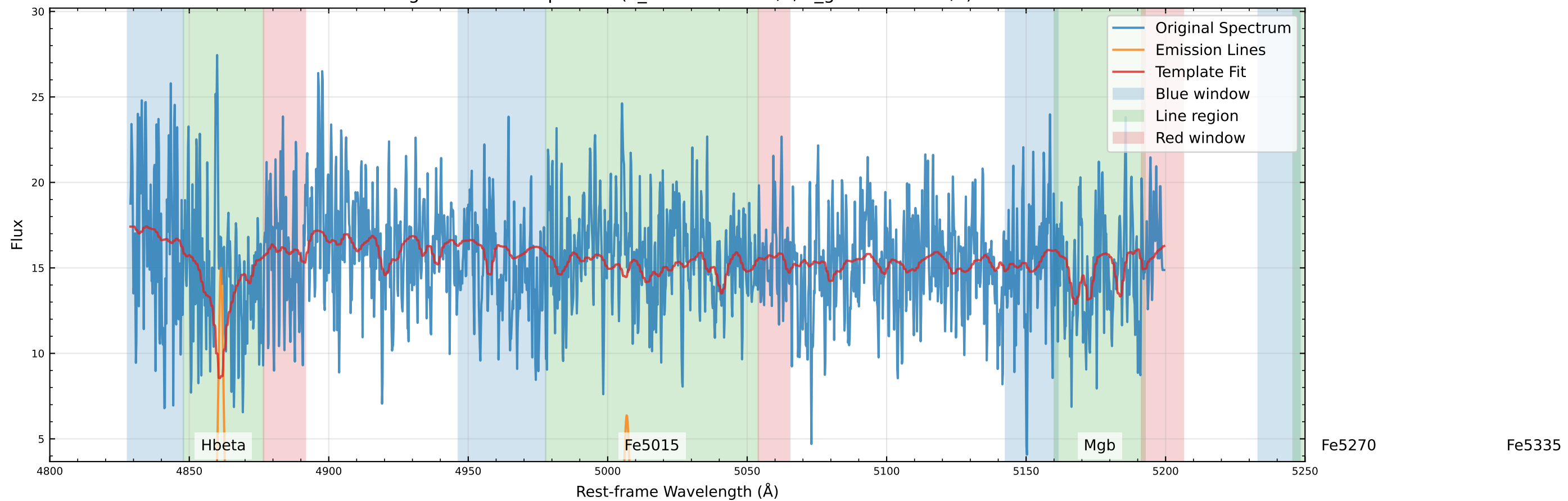
Original Data Comparison (v_star=-91.4 km/s, v_gas=-87.1 km/s)
