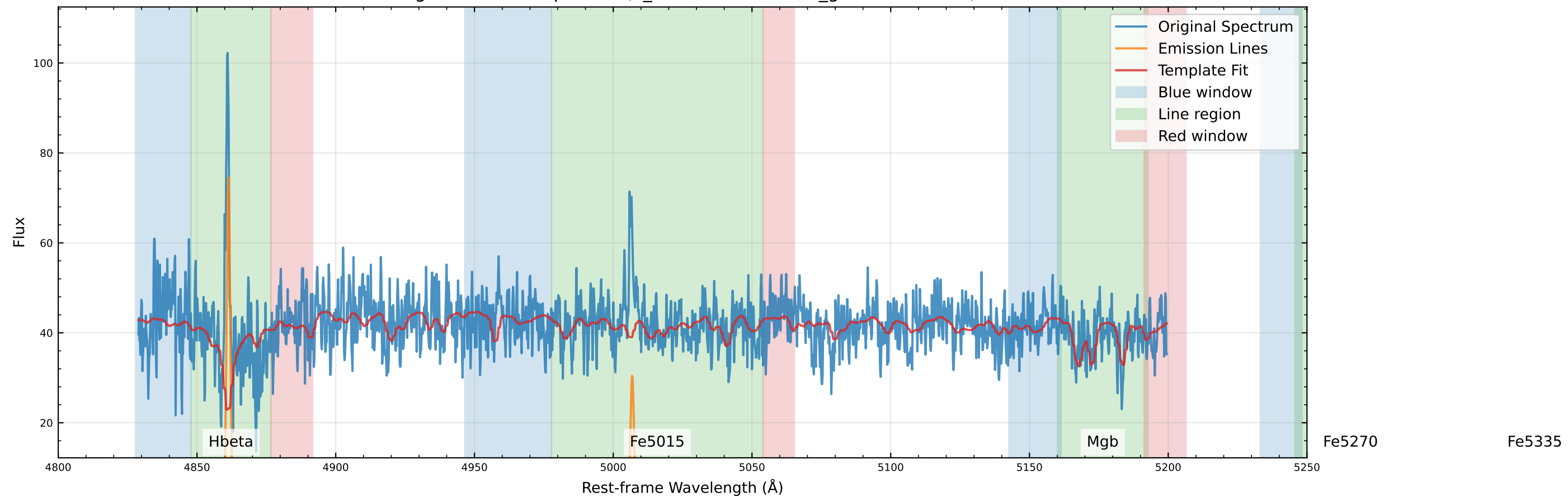
Original Data Comparison (v_star=-23.2 km/s, v_gas=-23.8 km/s)
