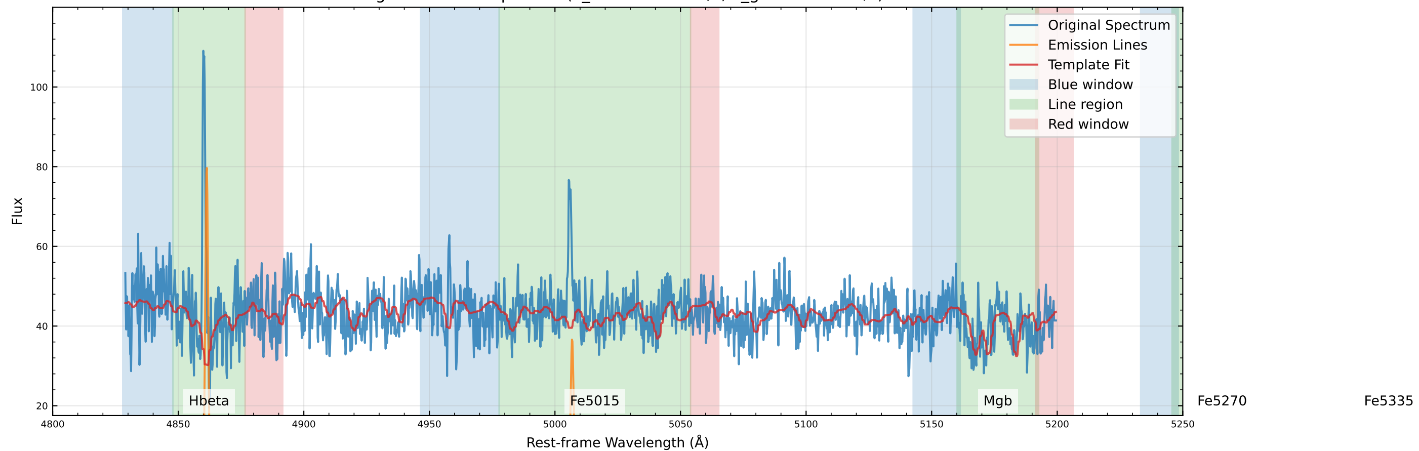
Original Data Comparison (v_star=-90.6 km/s, v_gas=-66.9 km/s)
