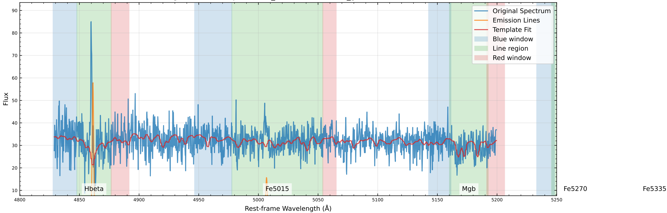
Original Data Comparison (v_star=-84.2 km/s, v_gas=-85.9 km/s)
