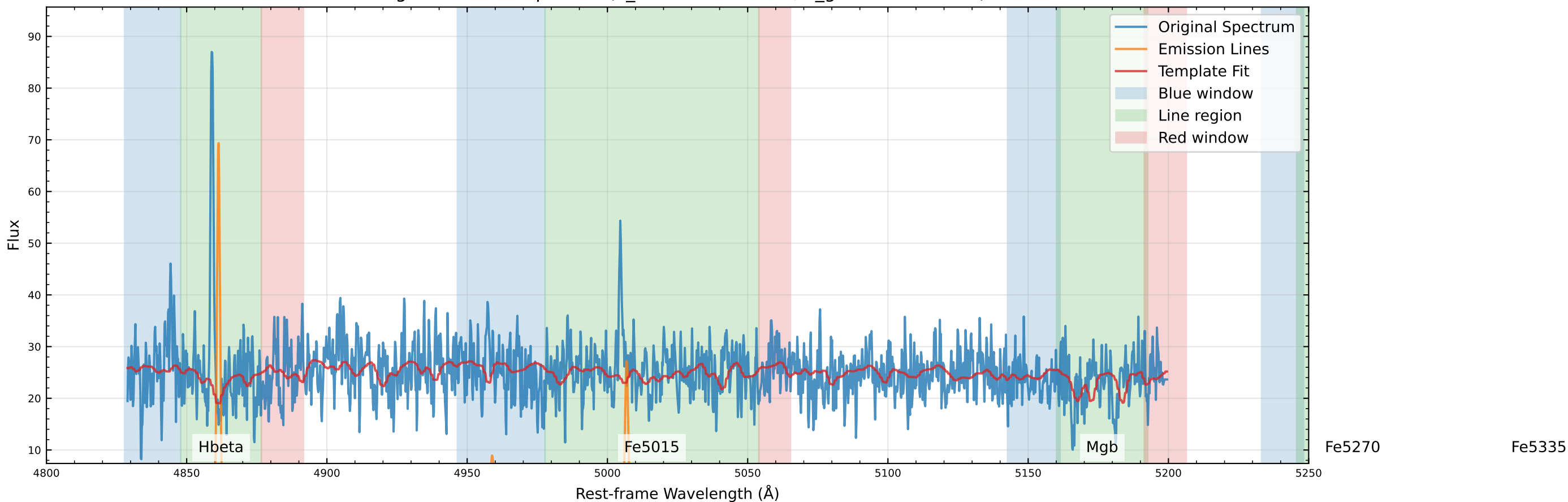
Original Data Comparison (v_star=-117.1 km/s, v_gas=-140.2 km/s)
