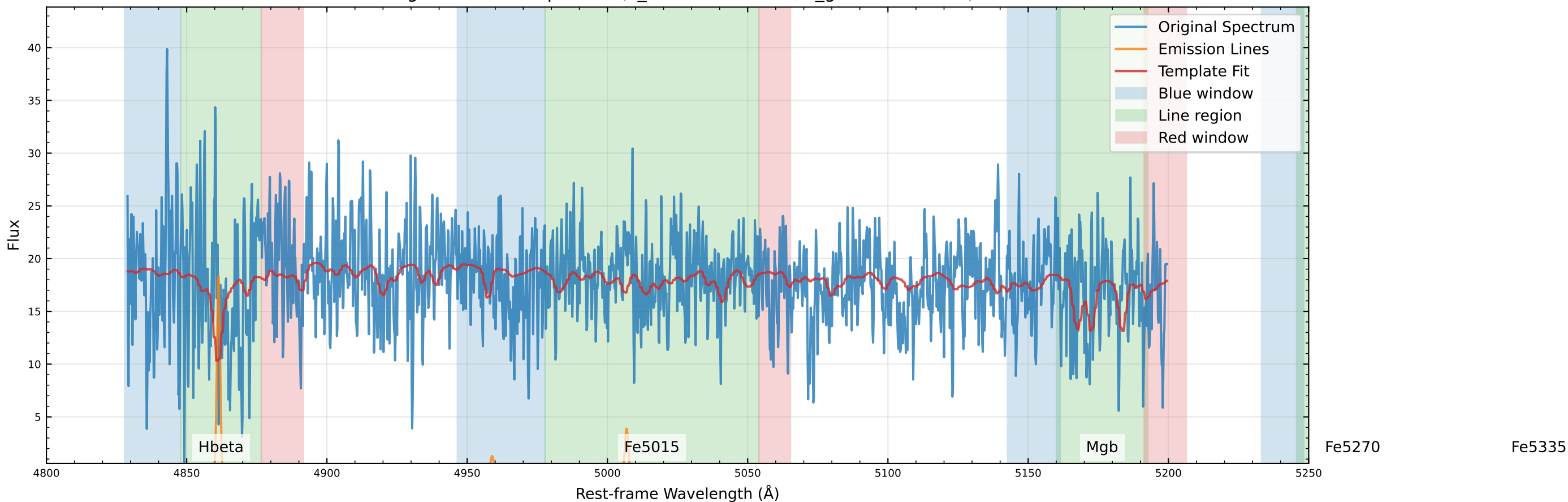
Original Data Comparison (v_star=-72.5 km/s, v_gas=-73.0 km/s)
