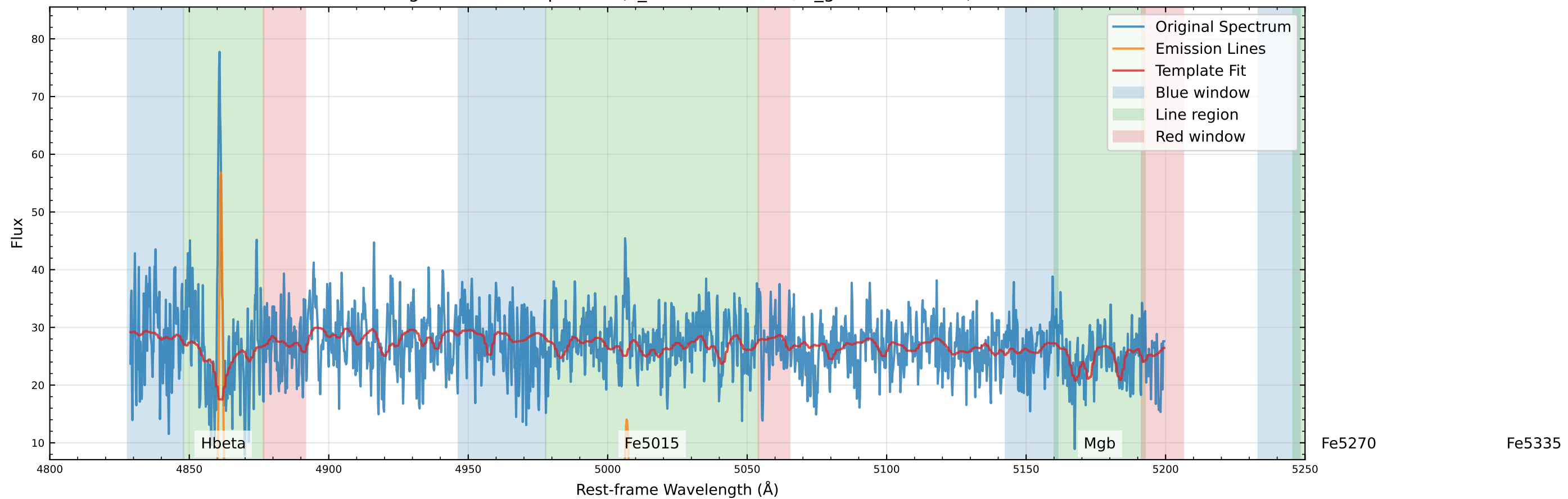
Original Data Comparison (v_star=-47.9 km/s, v_gas=-30.2 km/s)
