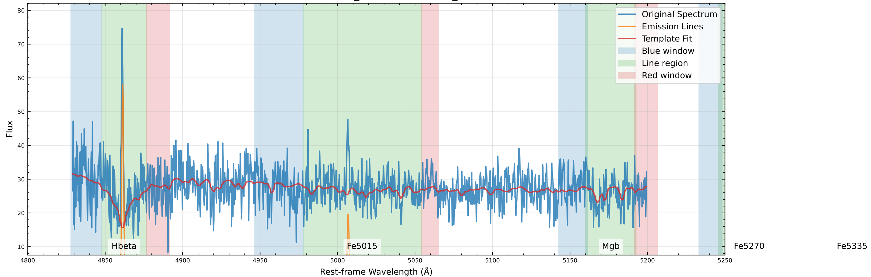
Original Data Comparison (v_star=-31.7 km/s, v_gas=-21.2 km/s)
