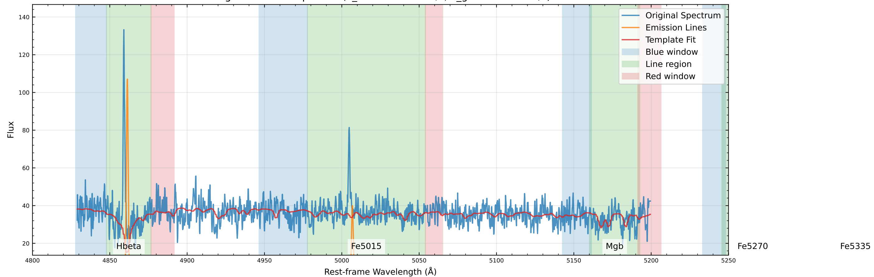
Original Data Comparison (v_star=-120.5 km/s, v_gas=-133.1 km/s)
