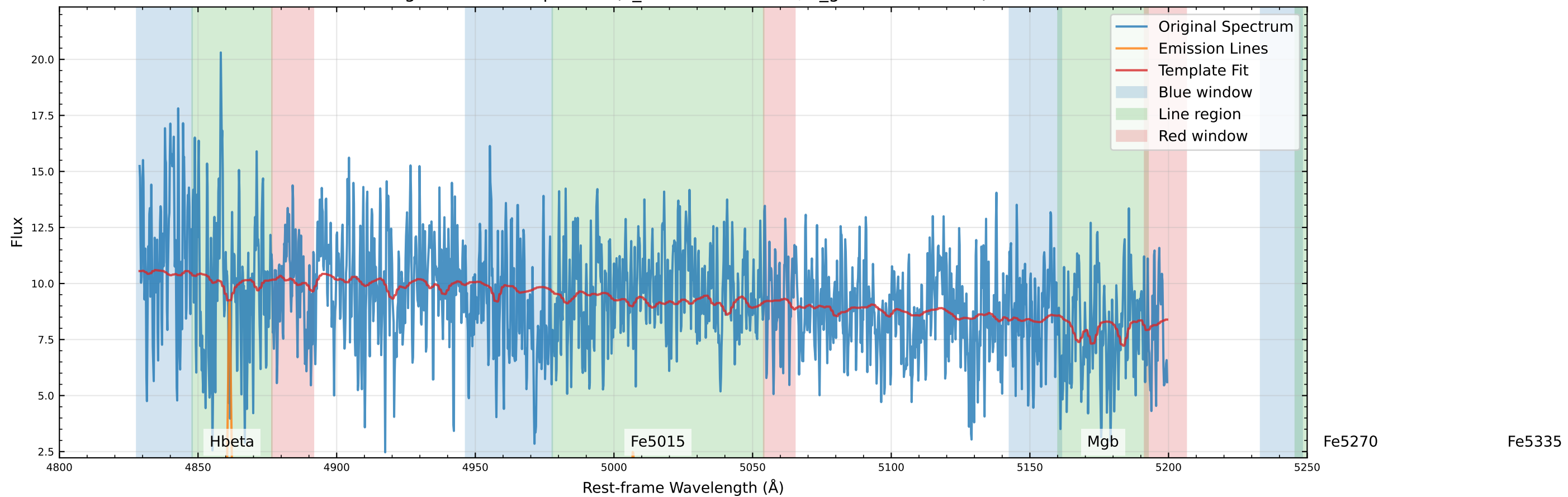
Original Data Comparison (v_star=-177.0 km/s, v_gas=-185.6 km/s)
