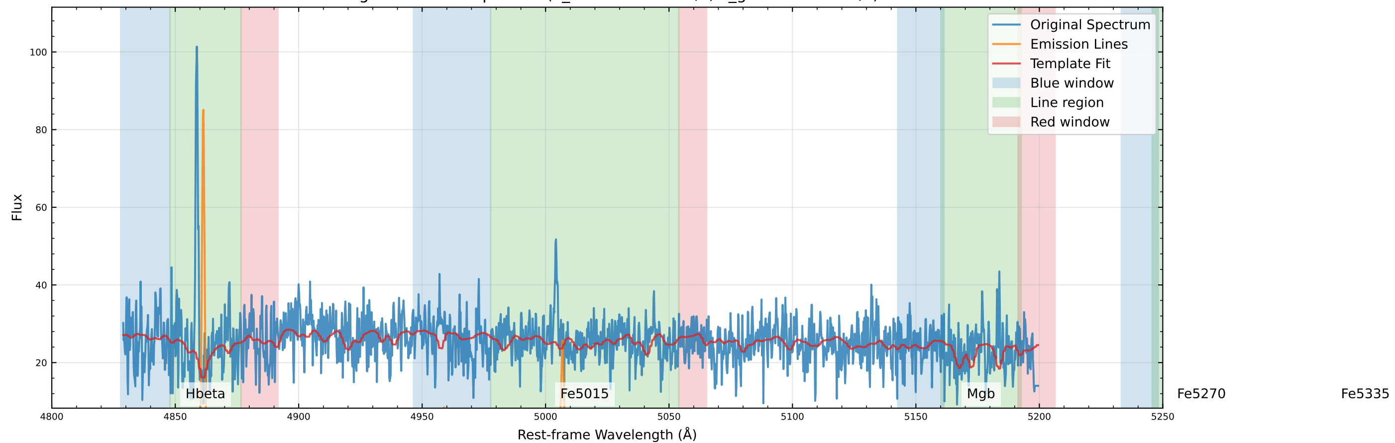
Original Data Comparison (v_star=-152.7 km/s, v_gas=-160.7 km/s)
