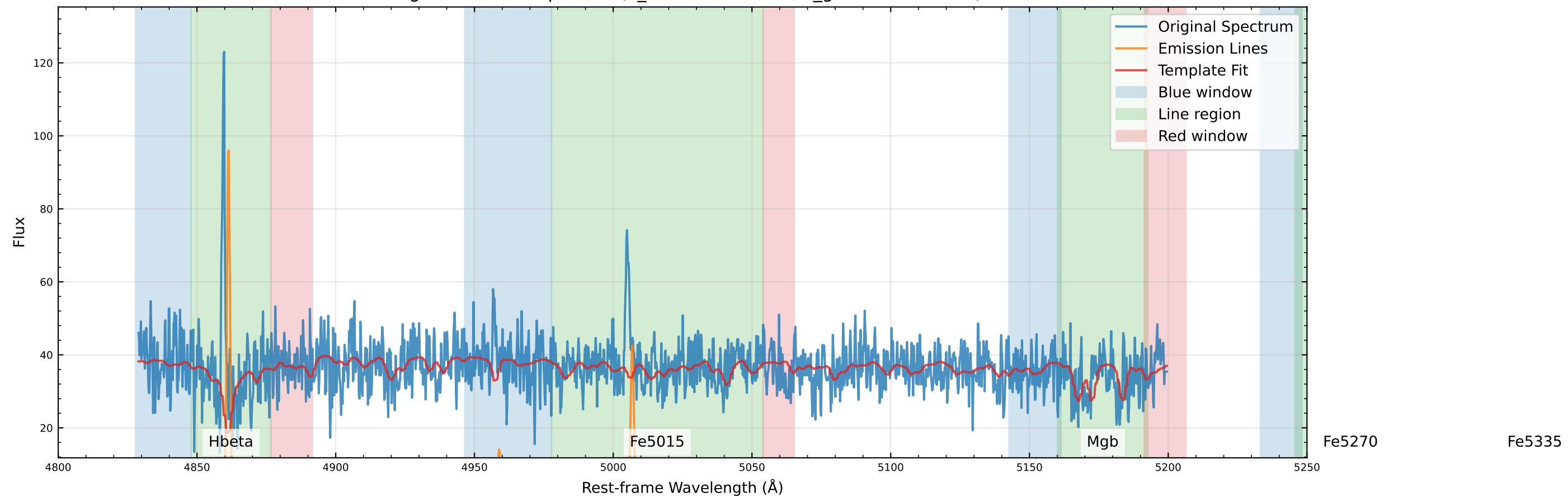
Original Data Comparison (v_star=-85.6 km/s, v_gas=-110.0 km/s)
