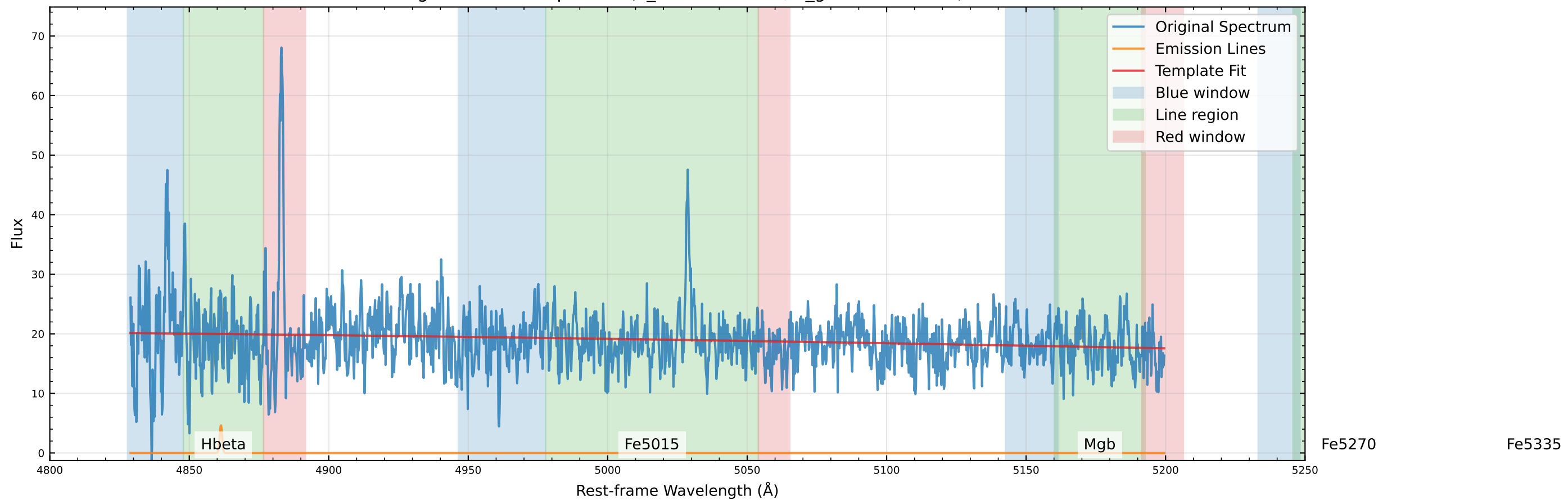
Original Data Comparison (v_star=0.0 km/s, v_gas=-16.1 km/s)
