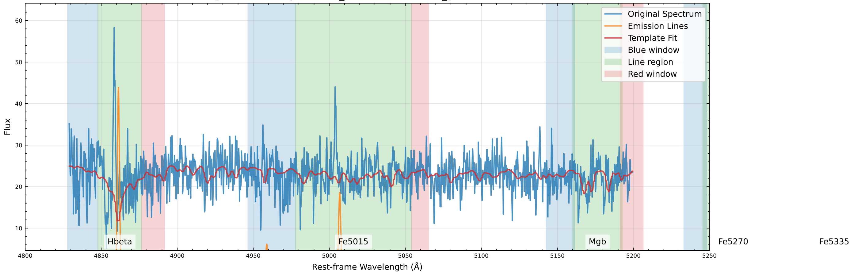
Original Data Comparison (v_star=-162.9 km/s, v_gas=-169.0 km/s)
