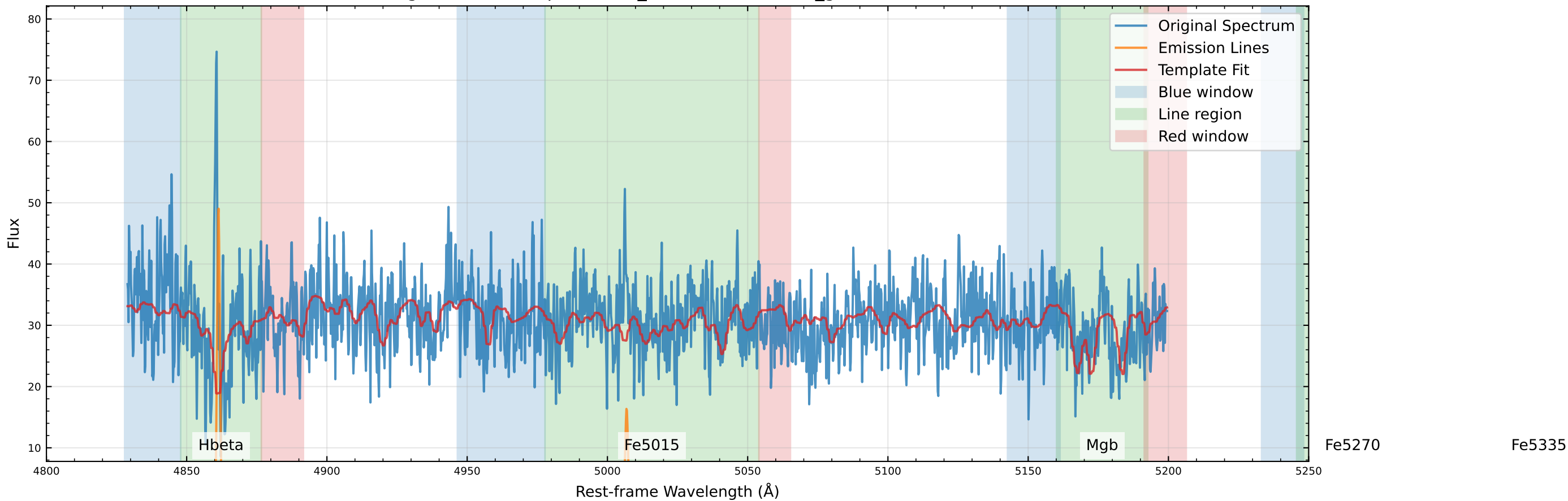
Original Data Comparison (v_star=-45.7 km/s, v_gas=-53.0 km/s)
