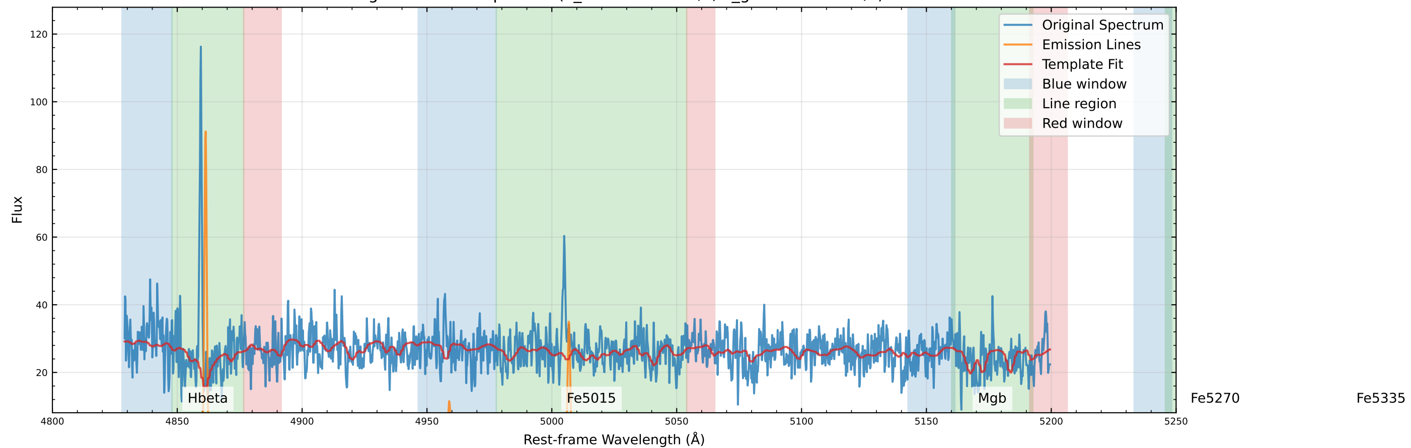
Original Data Comparison (v_star=-53.5 km/s, v_gas=-119.3 km/s)
