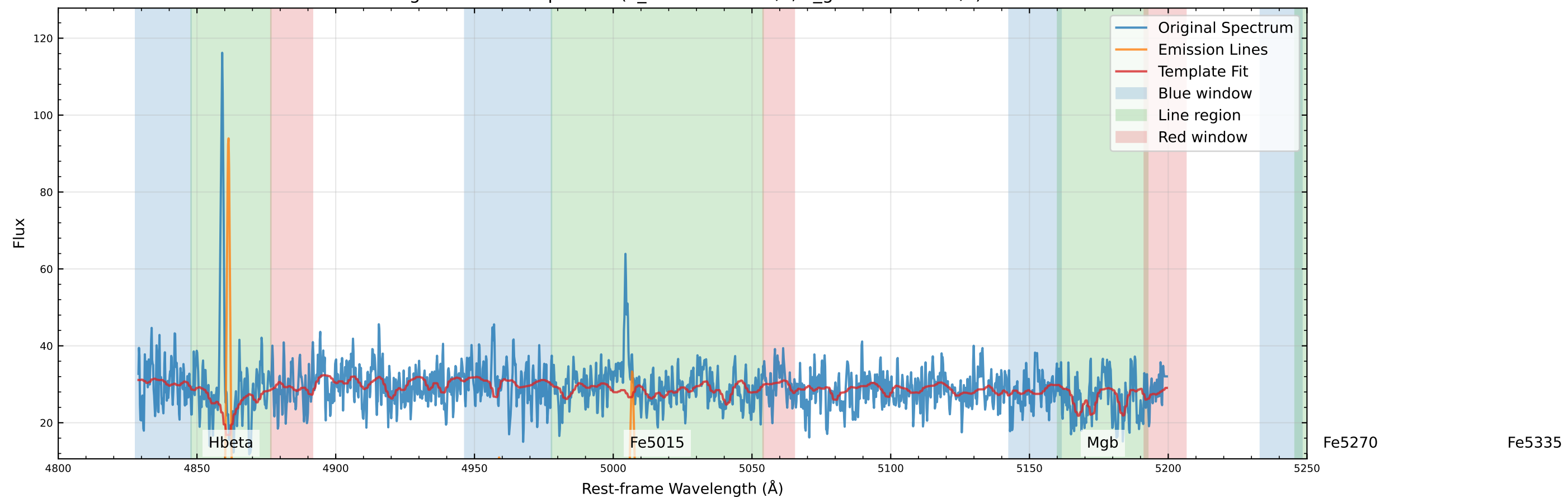
Original Data Comparison (v_star=-95.6 km/s, v_gas=-140.8 km/s)
