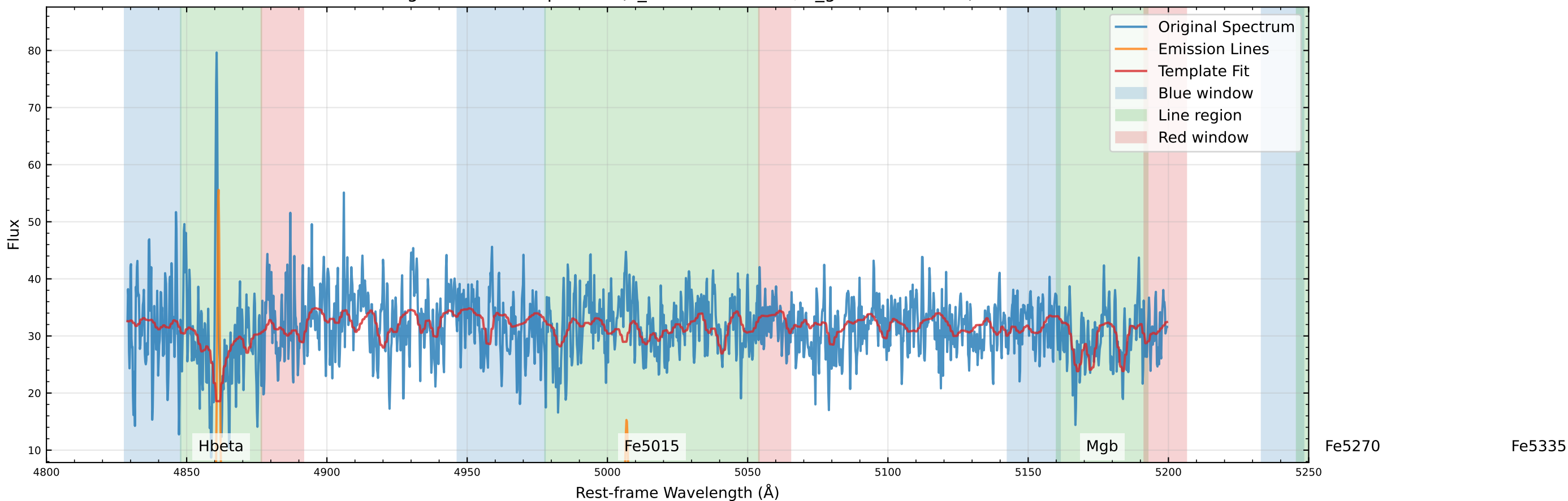
Original Data Comparison (v_star=-32.5 km/s, v_gas=-41.6 km/s)
