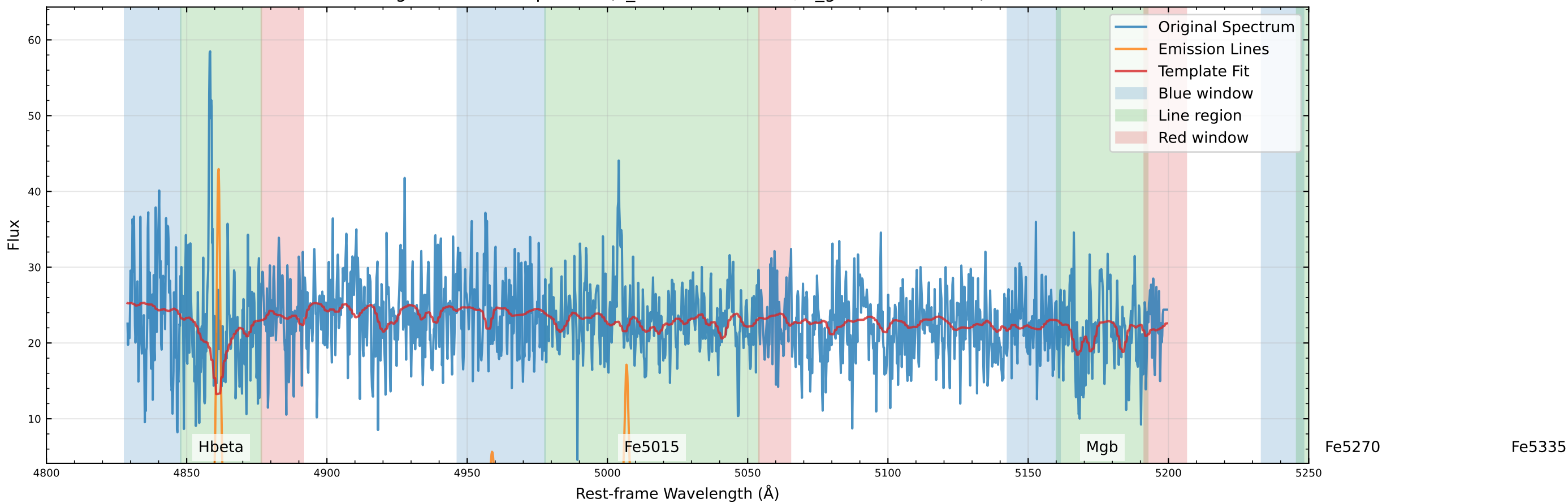
Original Data Comparison (v_star=-138.2 km/s, v_gas=-176.1 km/s)
