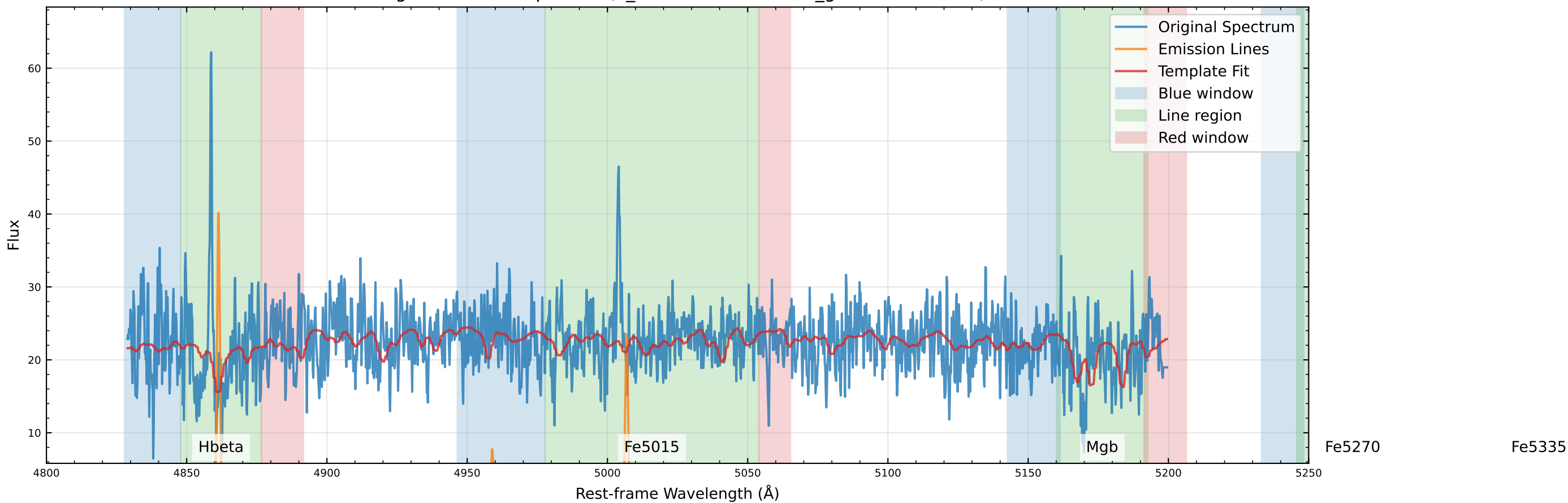
Original Data Comparison (v_star=-166.7 km/s, v_gas=-167.9 km/s)
