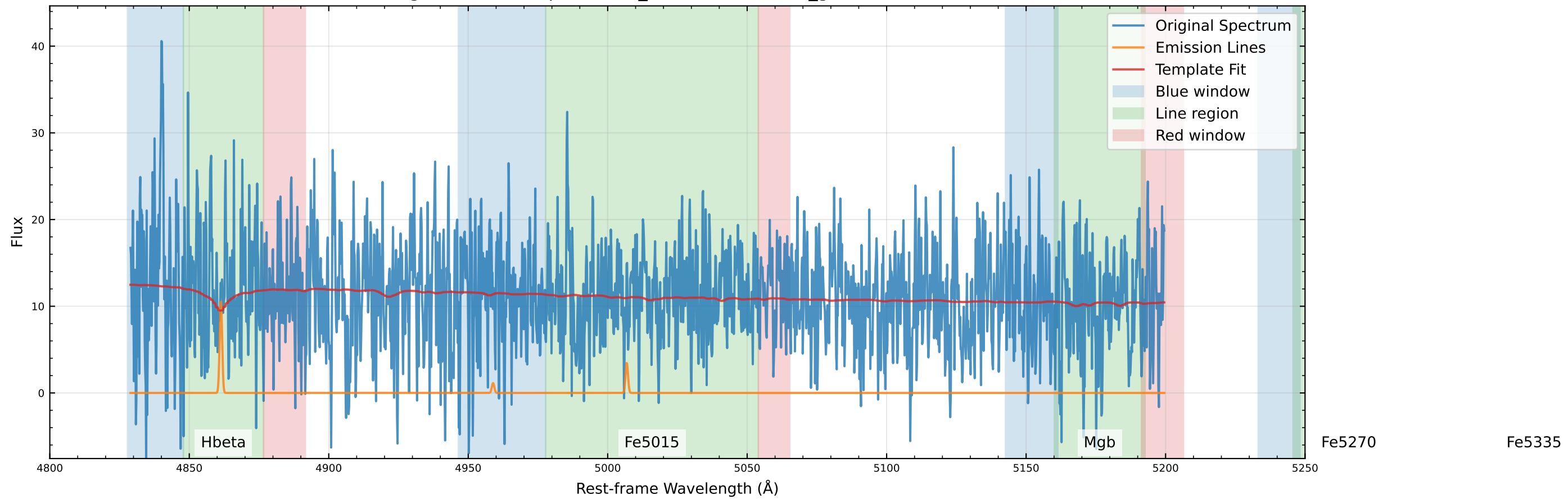
Original Data Comparison (v_star=44.2 km/s, v_gas=104.5 km/s)
