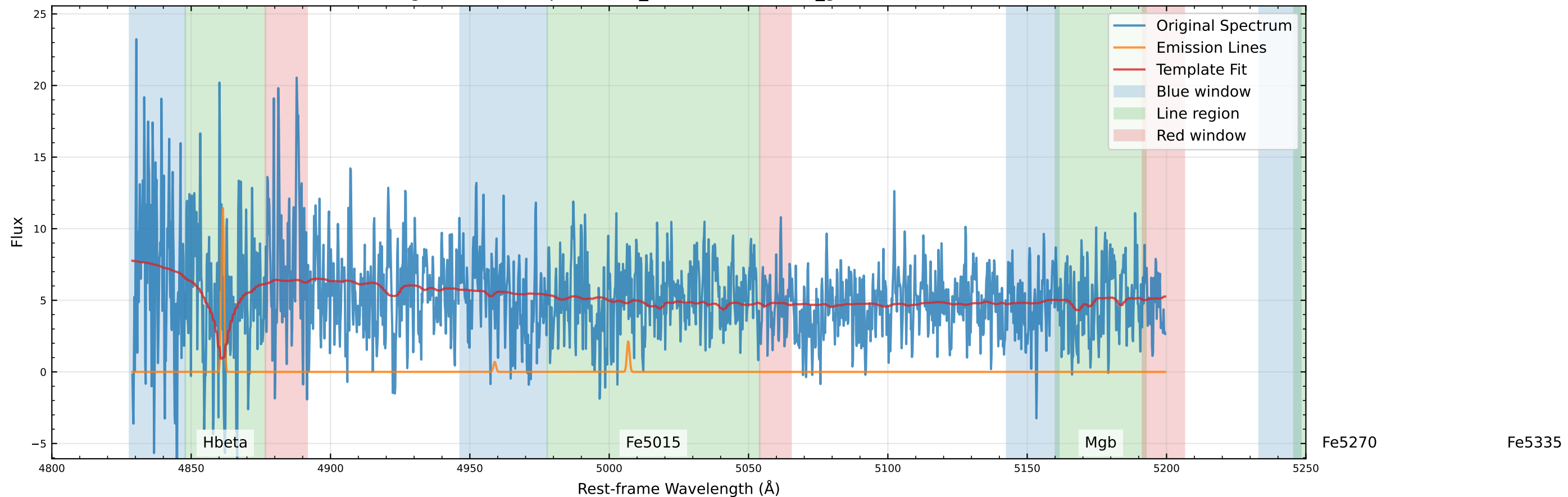
Original Data Comparison (v_star=-26.7 km/s, v_gas=-55.8 km/s)
