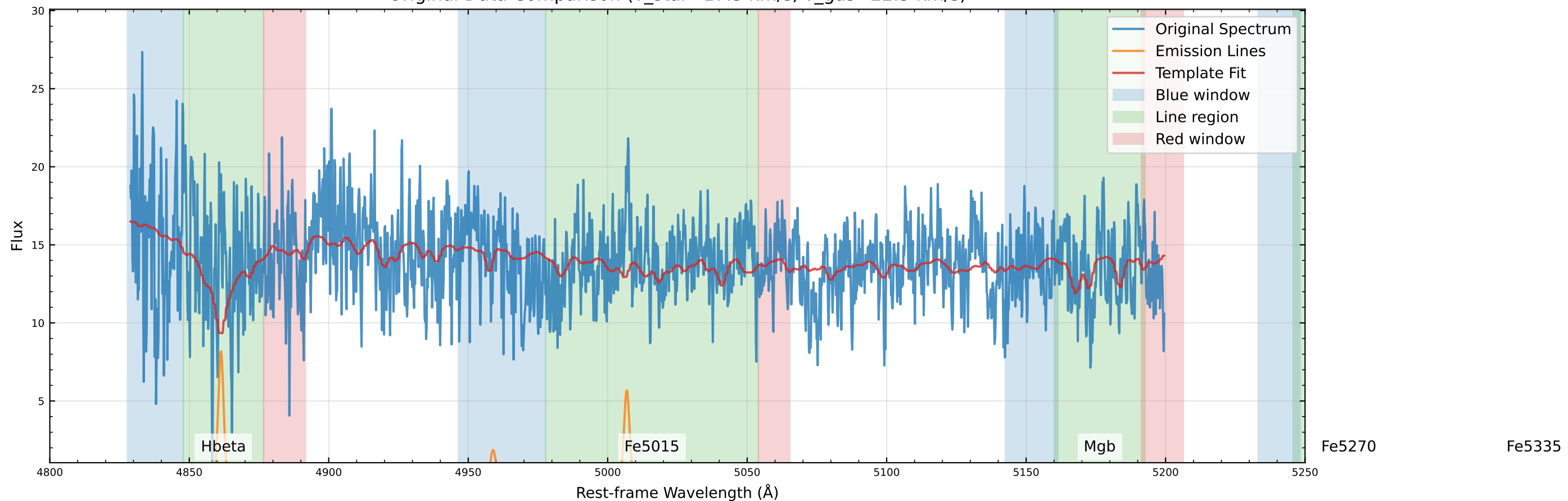
Original Data Comparison (v_star=17.3 km/s, v_gas=22.5 km/s)
