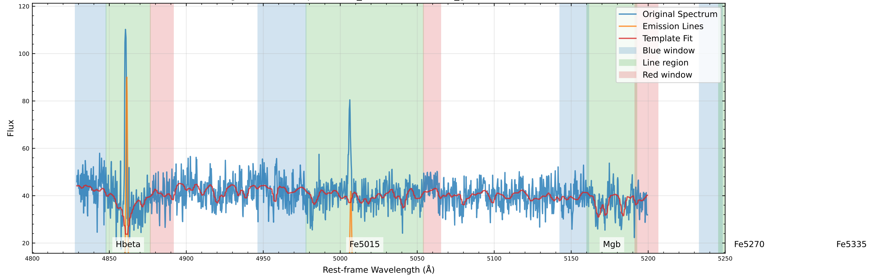
Original Data Comparison (v_star=-63.3 km/s, v_gas=-49.5 km/s)
