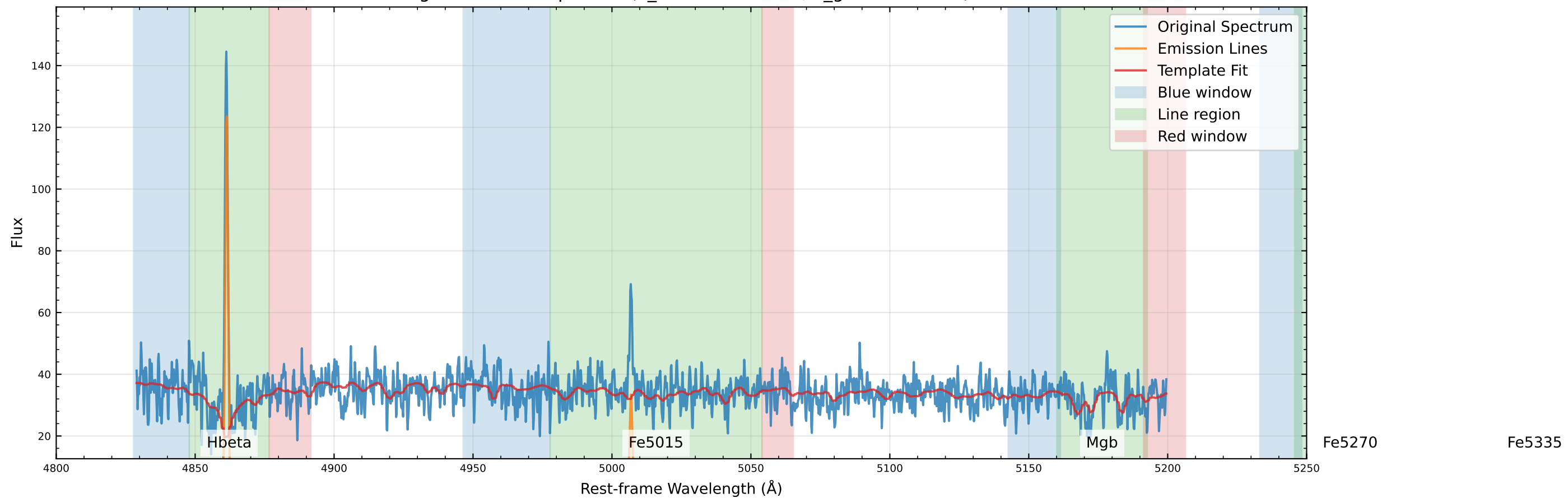
Original Data Comparison (v_star=-13.3 km/s, v_gas=-7.3 km/s)
