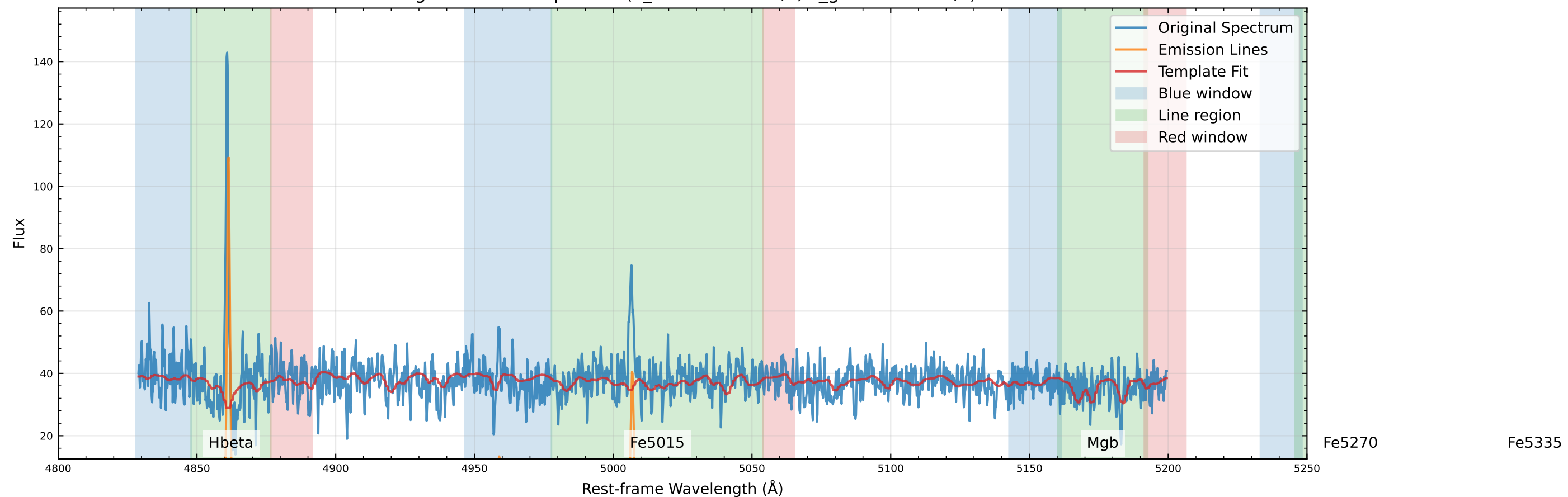
Original Data Comparison (v_star=-50.9 km/s, v_gas=-28.4 km/s)
