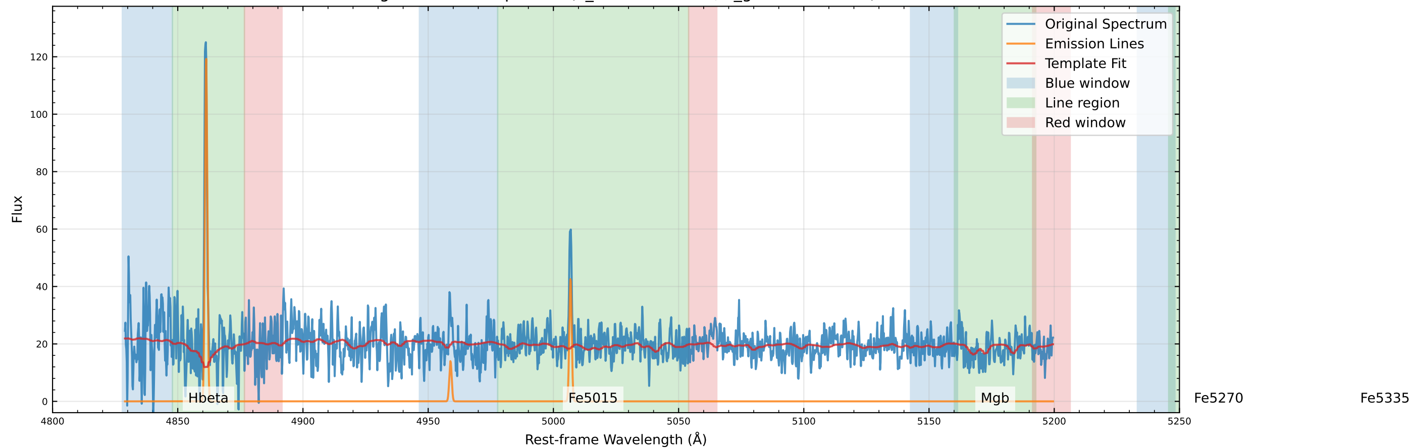
Original Data Comparison (v_star=-8.3 km/s, v_gas=-11.1 km/s)
