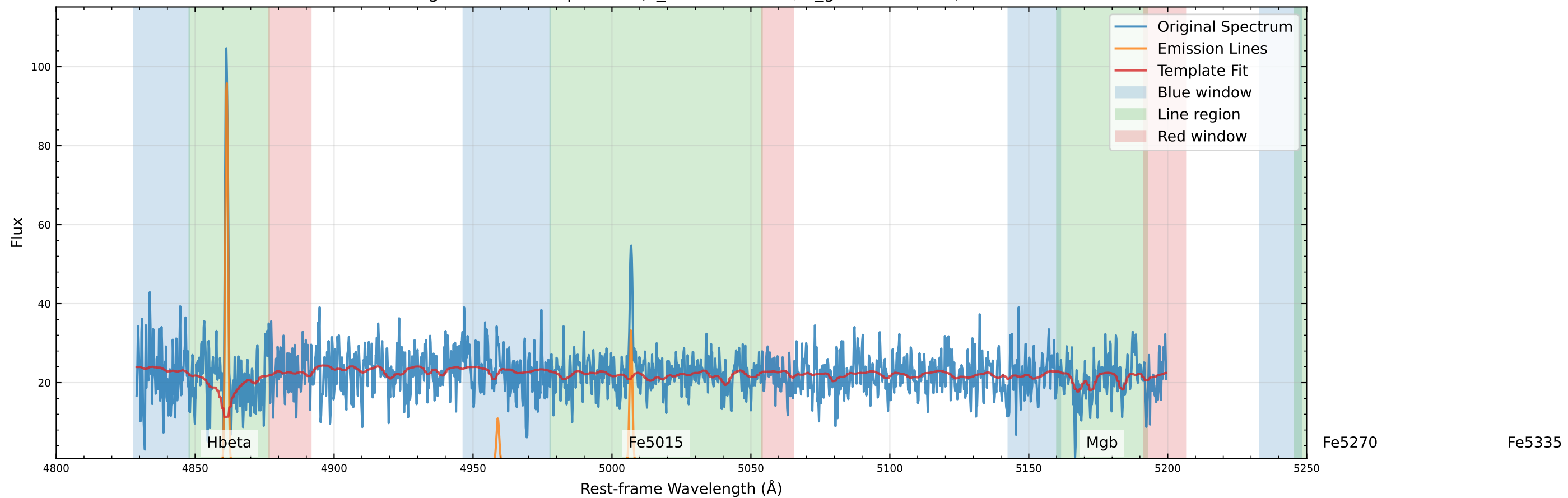
Original Data Comparison (v_star=5.7 km/s, v_gas=-0.8 km/s)
