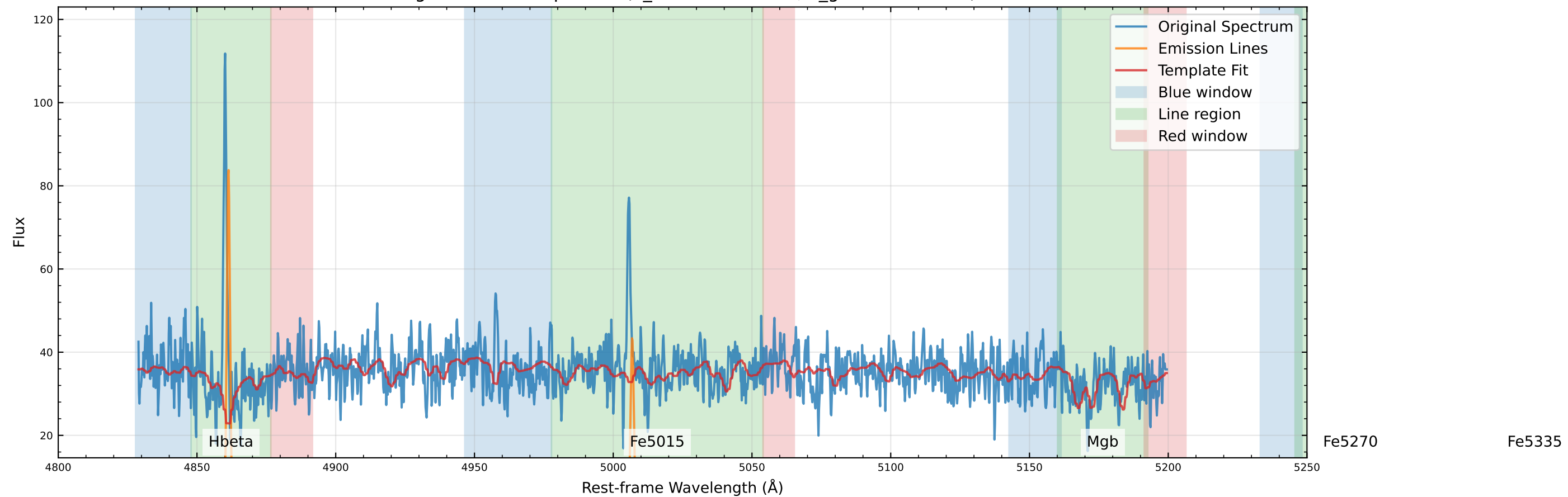
Original Data Comparison (v_star=-86.5 km/s, v_gas=-74.0 km/s)
