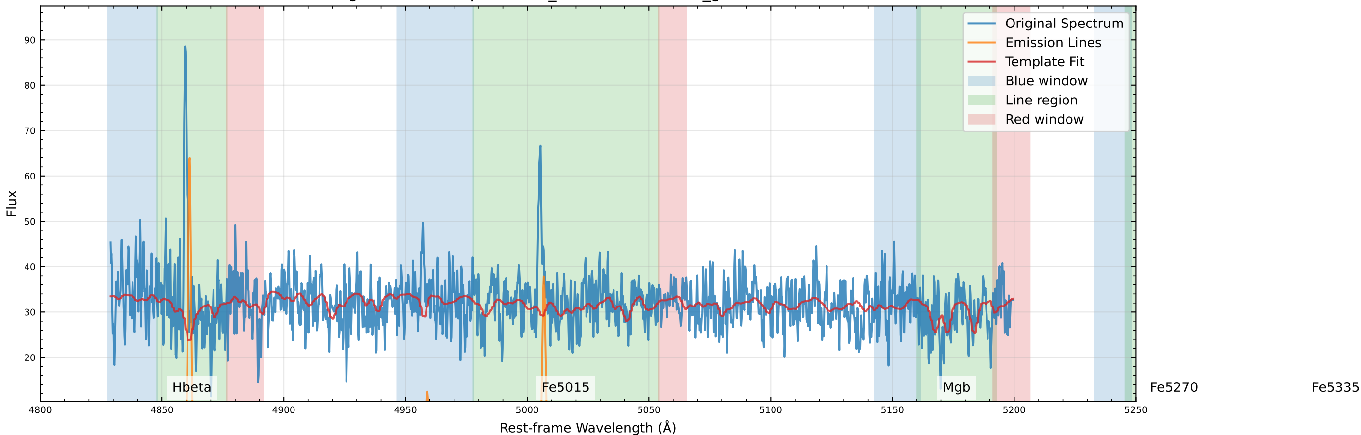
Original Data Comparison (v_star=-97.6 km/s, v_gas=-101.2 km/s)
