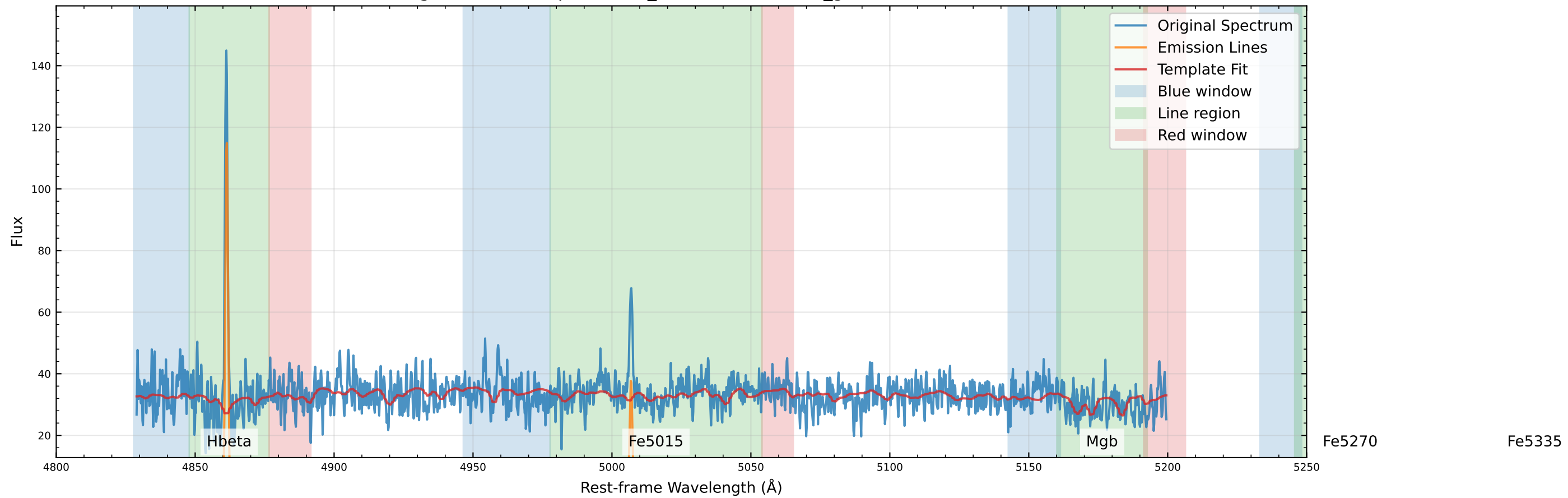
Original Data Comparison ( v_{\text{star}}=-16.1 km/s, v_{\text{gas}}=-8.1 km/s)
