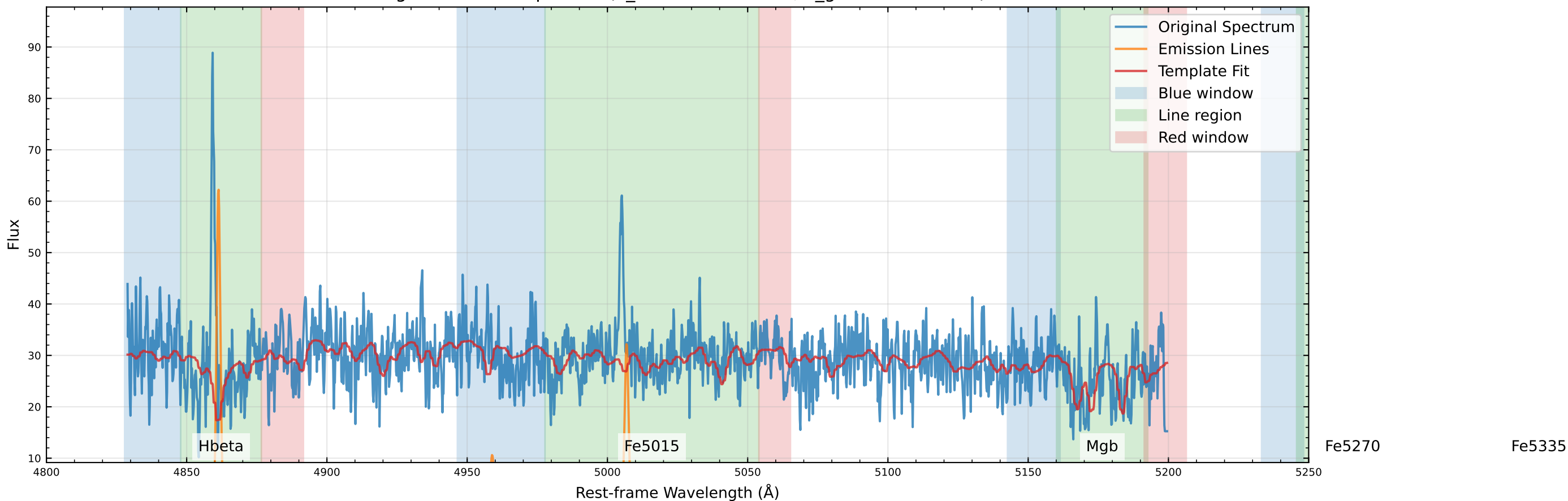
Original Data Comparison (v_star=-104.2 km/s, v_gas=-117.9 km/s)
