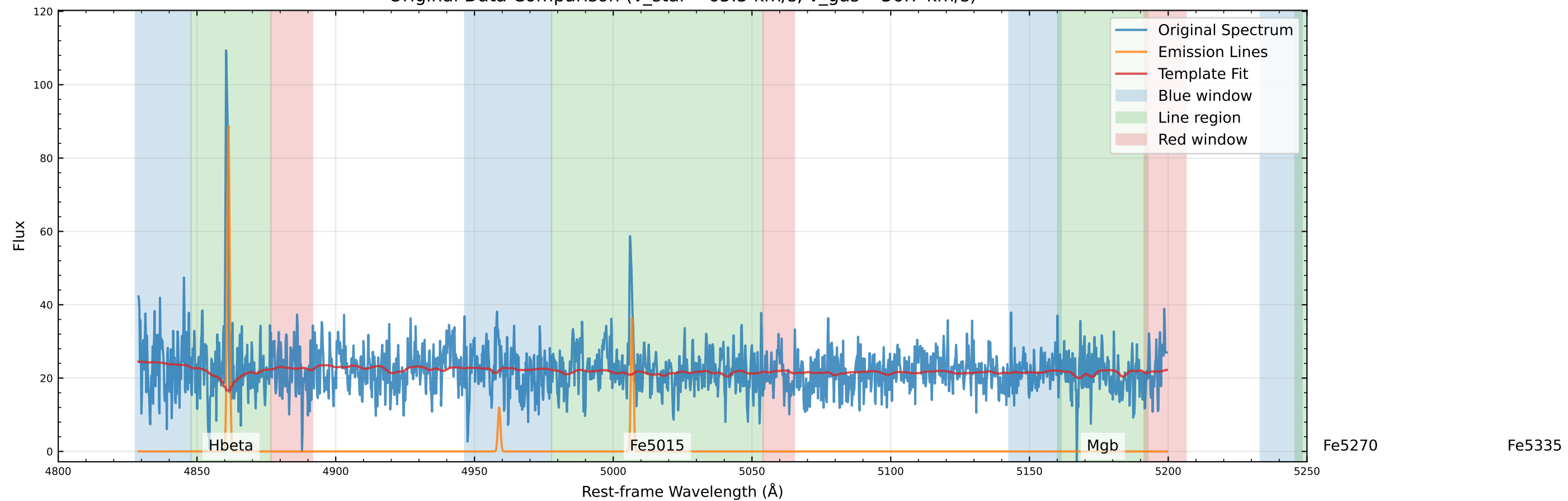
Original Data Comparison (v_star=-65.5 km/s, v_gas=-36.7 km/s)
