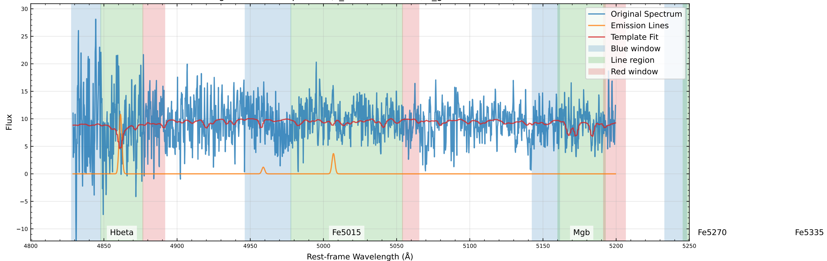
Original Data Comparison (v_star=-21.4 km/s, v_gas=-96.8 km/s)
