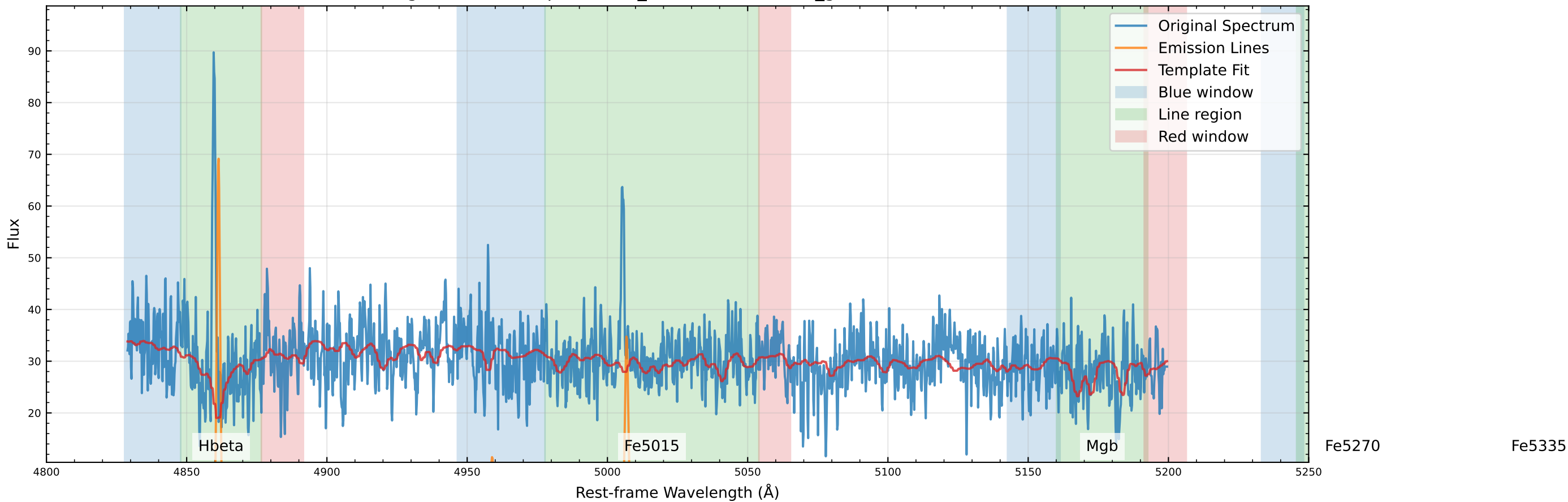
Original Data Comparison (v_star=-94.6 km/s, v_gas=-95.6 km/s)
