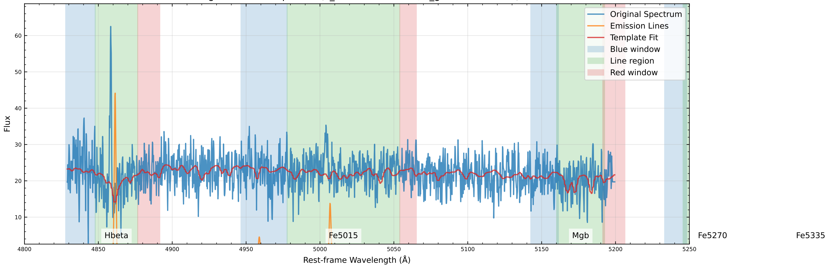
Original Data Comparison (v_star=-186.7 km/s, v_gas=-183.0 km/s)
