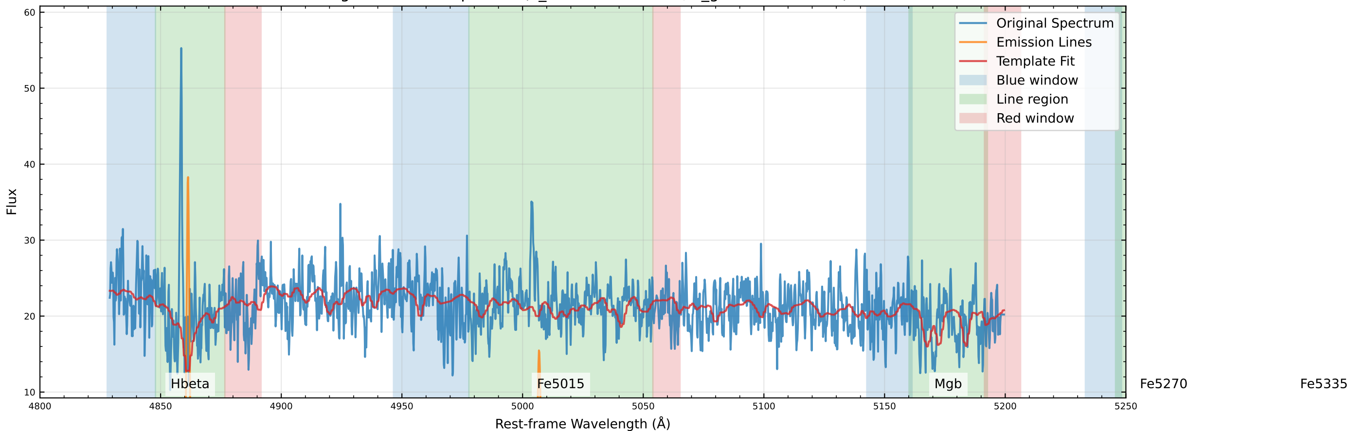
Original Data Comparison (v_star=-165.6 km/s, v_gas=-177.3 km/s)
