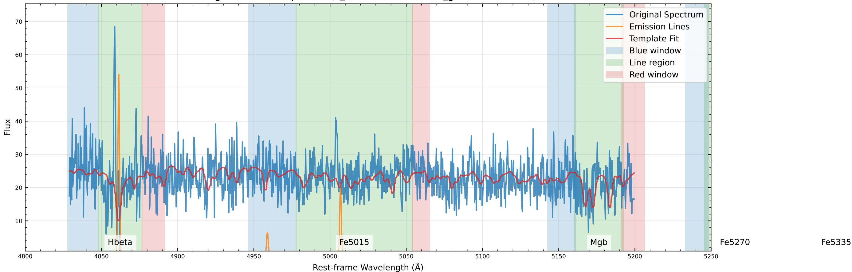
Original Data Comparison (v_star=-175.8 km/s, v_gas=-166.8 km/s)
