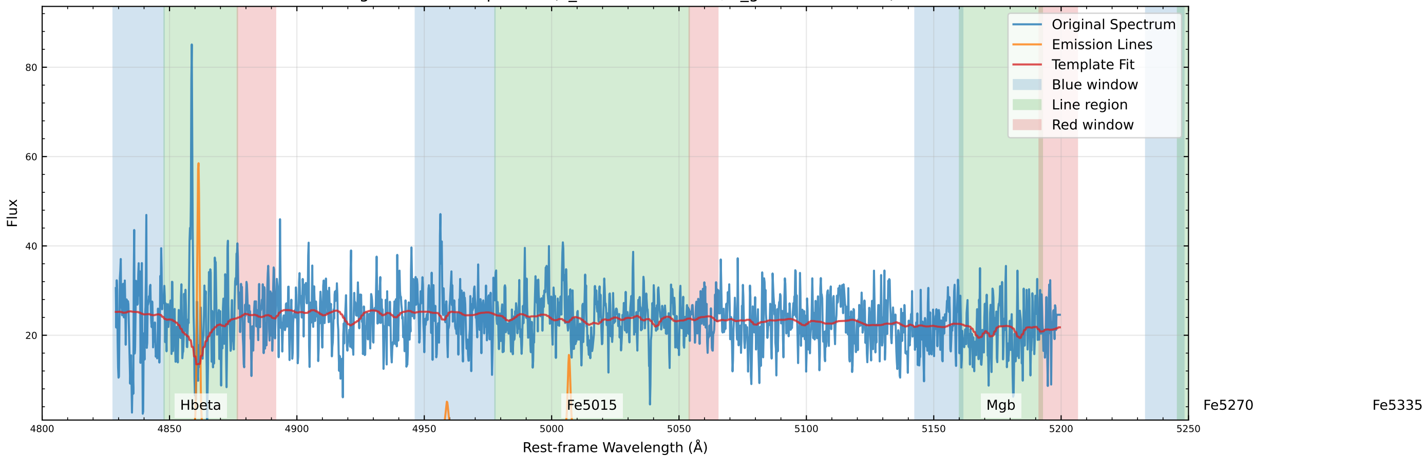
Original Data Comparison (v_star=-168.3 km/s, v_gas=-164.9 km/s)
