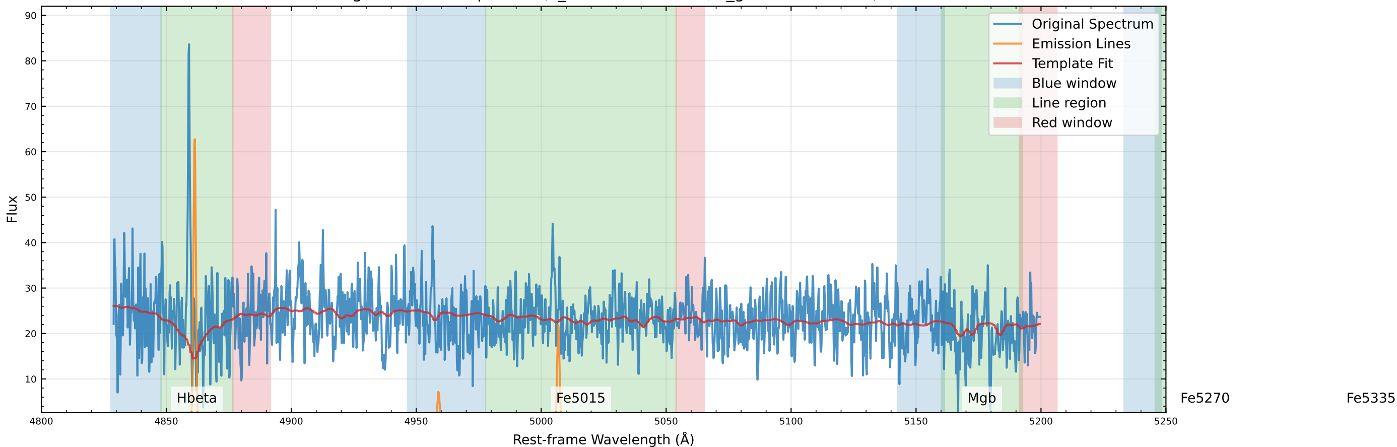
Original Data Comparison (v_star=-118.3 km/s, v_gas=-140.2 km/s)
