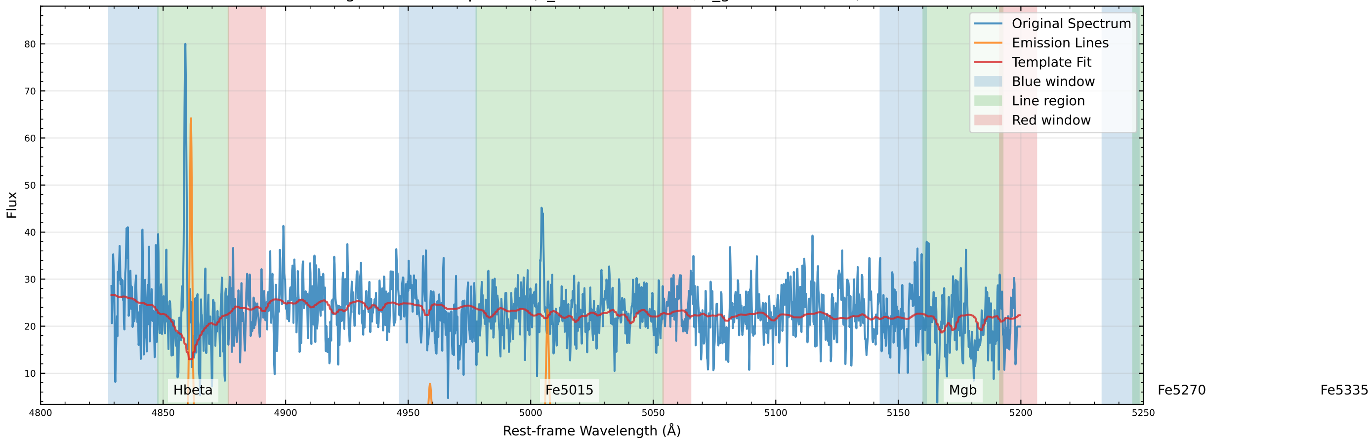
Original Data Comparison (v_star=-125.1 km/s, v_gas=-139.5 km/s)
