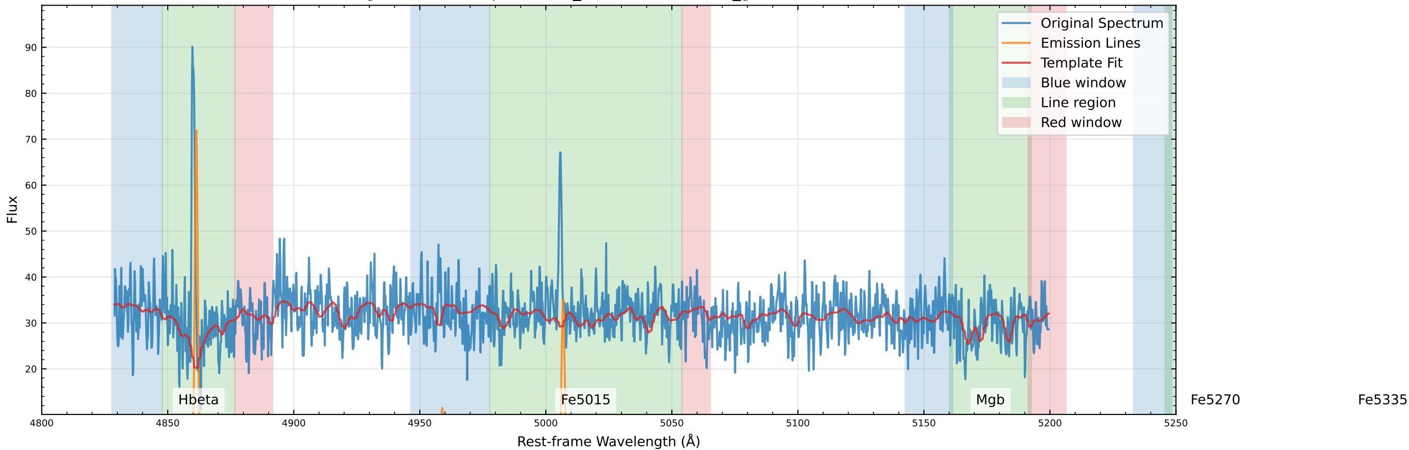
Original Data Comparison (v_star=-82.3 km/s, v_gas=-74.8 km/s)
