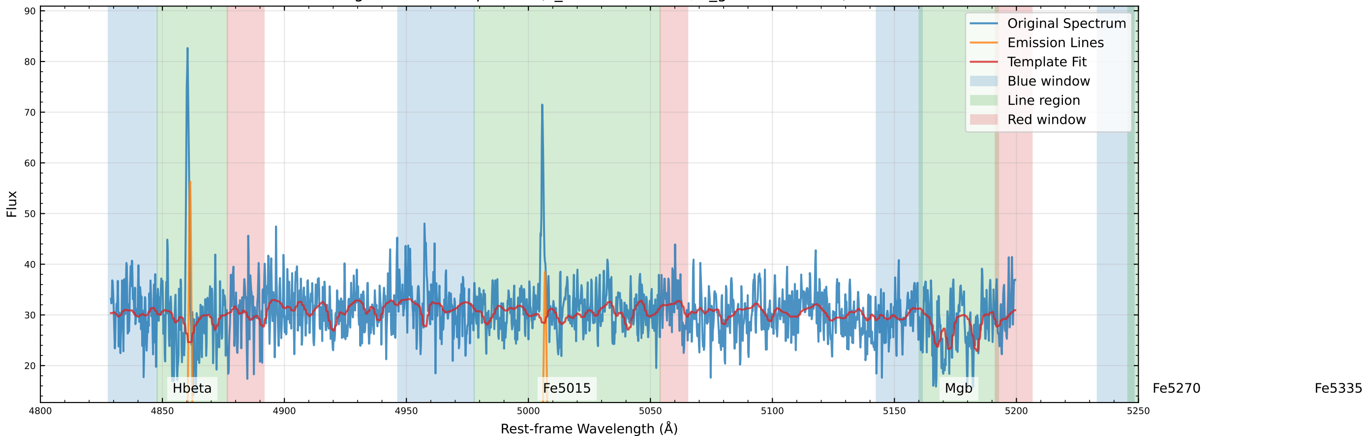
Original Data Comparison (v_star=-60.8 km/s, v_gas=-63.1 km/s)
