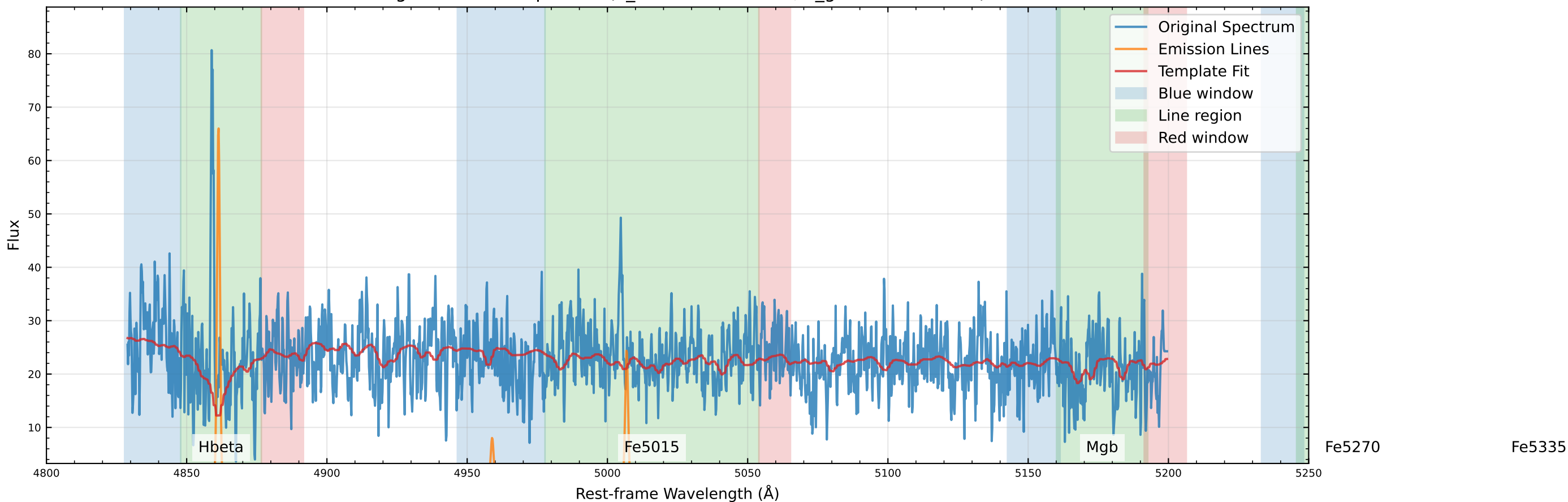
Original Data Comparison (v_star=-127.2 km/s, v_gas=-136.9 km/s)
