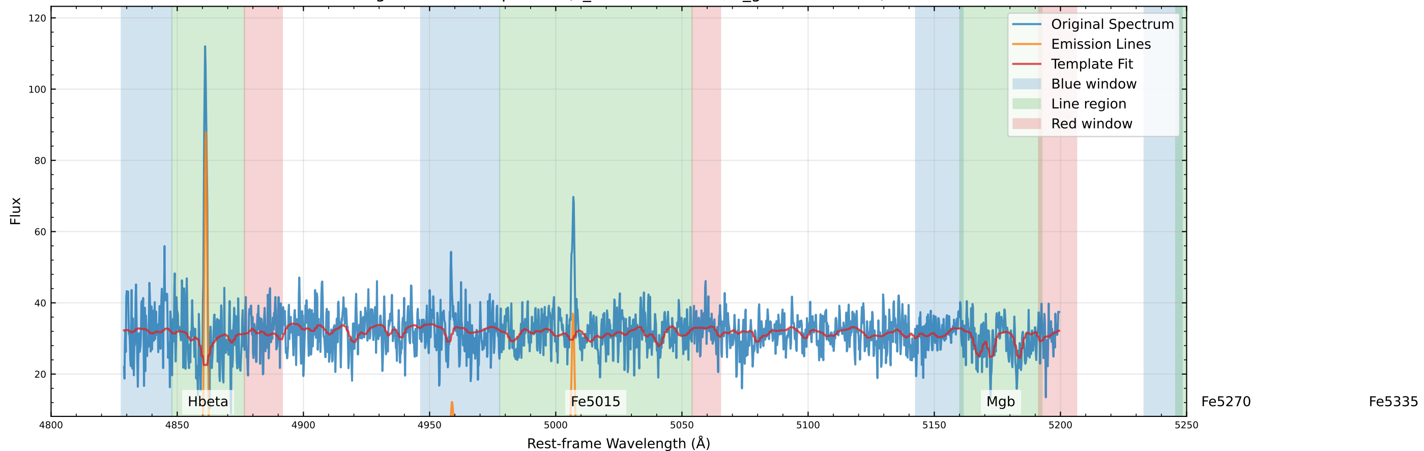
Original Data Comparison (v_star=-25.0 km/s, v_gas=-10.2 km/s)
