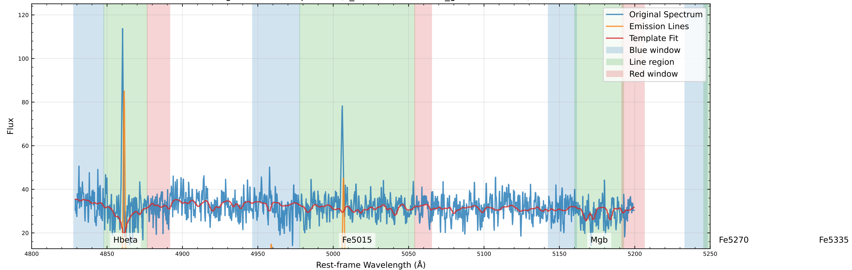
Original Data Comparison (v_star=-77.5 km/s, v_gas=-63.7 km/s)
