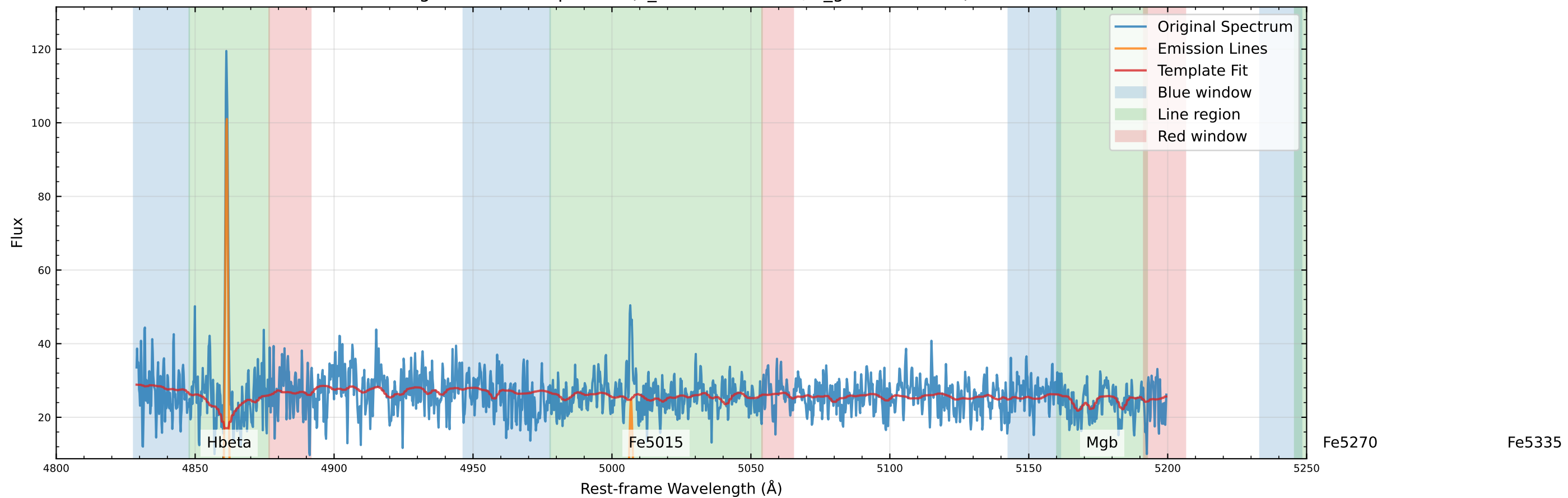
Original Data Comparison (v_star=-15.5 km/s, v_gas=-0.0 km/s)
